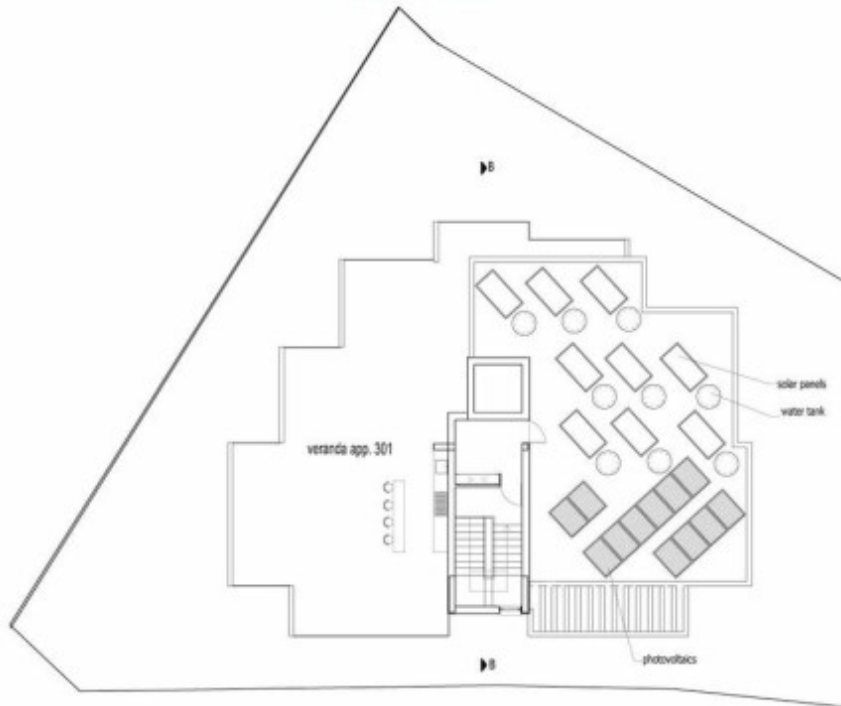
Roof Plan
