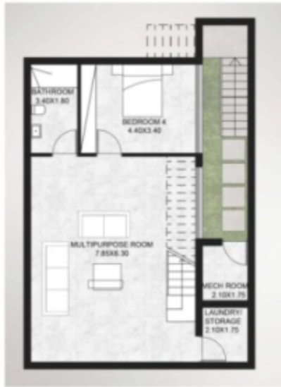
BASEMENT PLAN
