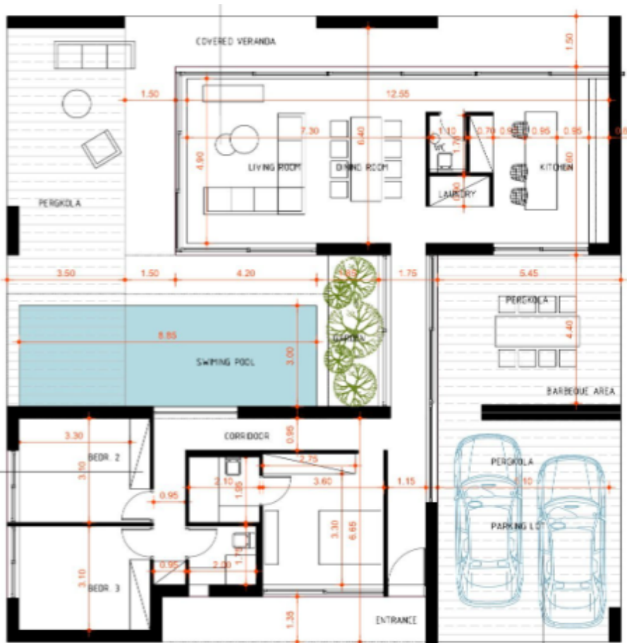
Ground Floor clasic Areas 160.50sqm Covered Areas 160.50sqm
