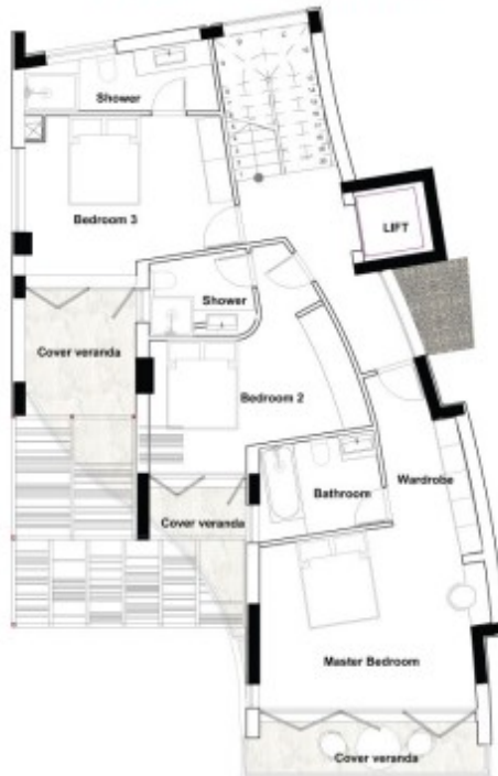
Villa 2 - First Floor Plan
