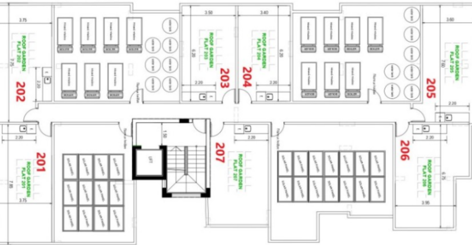
ROOF GARDEN PLAN
