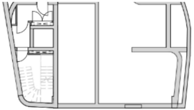
BASEMENT -2
